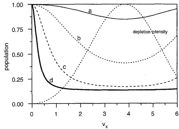
Fig. 3. The effect of the depletion beam h_{depl}(v) |_x (dashed) on the probability of the dye not to be in the triplet state, 1 - n_2(v) , for the maximum of h_{depl}(v) |_x of (a) 0.001, (b) 0.01, (c) 0.1 and (d) 1 MW/cm^2
