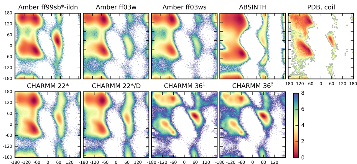
Figure 3. Force field differences in backbone dihedral angles. The potential of mean force (PMF), -\log(P(\varphi,\psi)) , with color scale in kT, is shown for each force field. The upper right graph (PDB, coil) corresponds to all non-Pro, non-Gly residues that are not in helix or sheet secondary structure in the TOP500 90 structures (a set of nonredundant protein structures from the PDB). The population in the \alpha L basin in each case is Amber ff99sb*-ildn = 0.12, Amber ff03w = 0.01, Amber ff03ws = 0.01, ABSINTH = 0.02, CHARMM 22* = 0.05, CHARMM 22* (with TIP4P-D) = 0.04, CHARMM 36 (with TIP3P) = 0.42, CHARMM 36 (with charmm-modified TIP3P) = 0.41, and PDB, coil = 0.06. More than 85% of conformations in the CHARMM 36 ensemble contain left-handed \alpha -helix. Refer to Figures S6 and S7 for the same analysis for arginine and serine residues separately.
