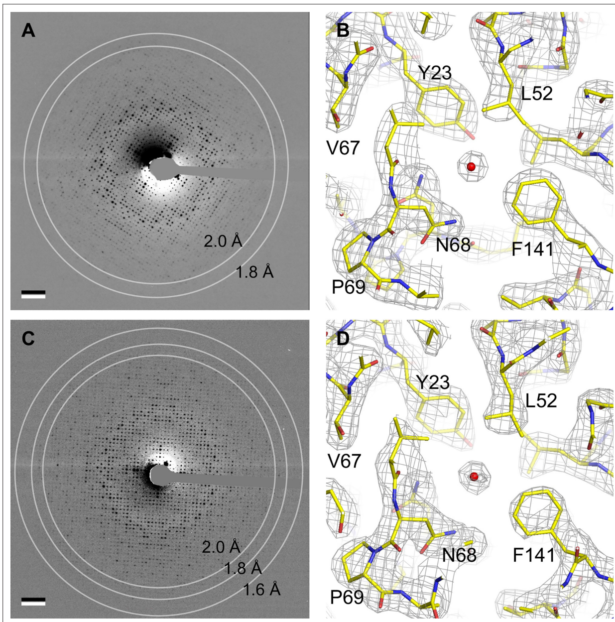
Figure 2. Electron crystallography provides structures of aquaporin-0 (AQP0) in sphingomyelin/ cholesterol bilayers at 2.5 Å resolution. (A) Electron diffraction pattern of an untilted AQP0 two-dimensional (2D) crystal reconstituted at a sphingomyelin:cholesterol ratio of 2:1, showing reflections to ~2 Å resolution. Scale bar indicates (10 \text{ \AA})^{-1} . (B) Density map at 2.5 Å resolution used to build the AQP0 2SM:1Chol structure. A region of the water-conducting pathway close to the NPA (asparagine-proline-alanine), the AQP signature motif, is shown. The 2F_o - F_c map contoured at 1.5\sigma is shown as gray mesh, the AQP0 model is shown in yellow with oxygen atoms in red and nitrogen atoms in blue. The red sphere represents a water molecule. (C) A diffraction pattern of an untilted AQP0 2D crystal reconstituted at a sphingomyelin:cholesterol ratio of 1:2, showing reflections to better than 1.6 Å resolution. Scale bar indicates (10 \text{ \AA})^{-1} . (D) Density map at 2.5 Å resolution used to build the AQP0 1SM:2Chol structure. The same region as in (B) is shown with the same color code. See also Figure 2—figure supplement 1 .
