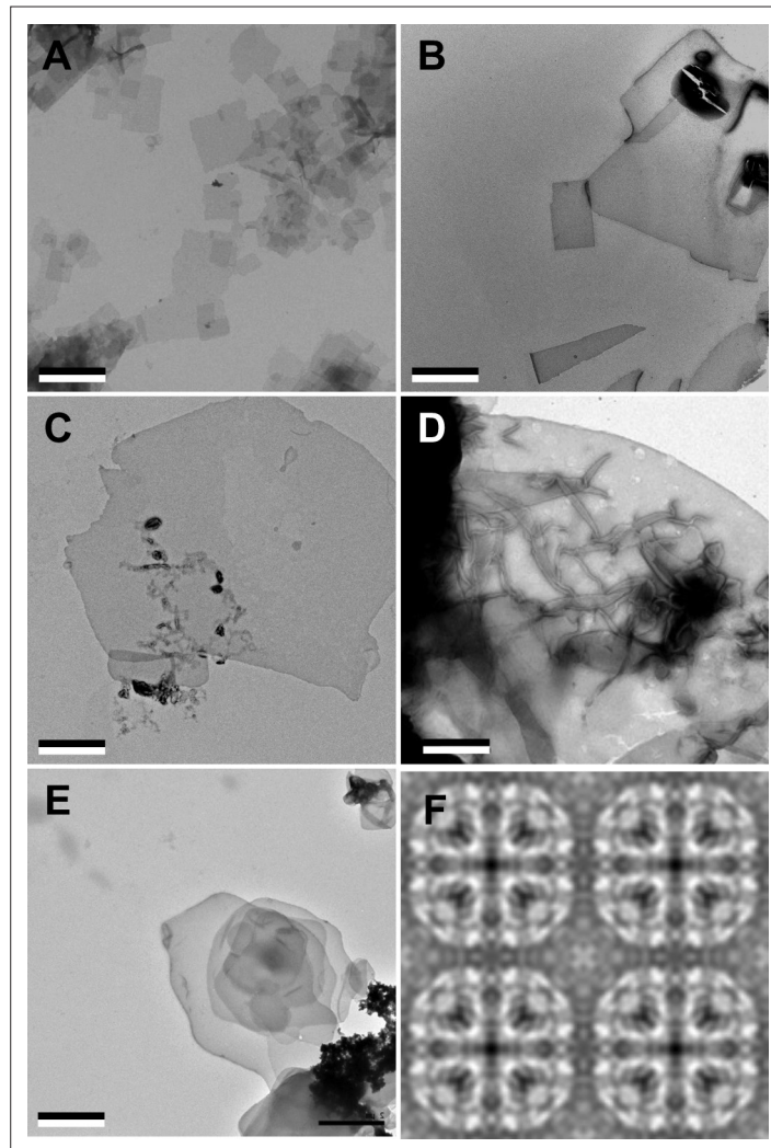
Figure 1. Aquaporin-0 (AQP0) forms two-dimensional (2D) crystals with all tested sphingomyelin/cholesterol mixtures. (A–E) AQP0 purified from sheep lenses was reconstituted with pure sphingomyelin (A), sphingomyelin/cholesterol mixtures at molar ratios of 2:1 (B), 1:2 (C), and 1:4 (D), as well as pure cholesterol (E). AQP0 was reconstituted under all conditions and formed diffracting 2D crystals. The scale bars are 2 \mu\text{m} . (F) Projection map of AQP0 reconstituted with pure cholesterol at 3.2 \text{\AA} resolution. The 2D crystals show p422 symmetry and have the typical lattice constants for AQP0 crystals of a=b=65.5 \text{ \AA} , and \gamma=90^\circ . The panel shows two-by-two unit cells. See also Figure 1—figure supplements 1 and 2 and Tables 1 and 2 .
