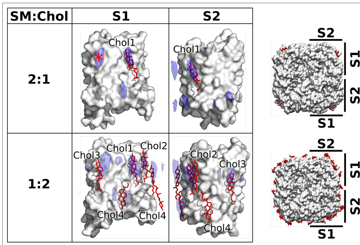
Figure 5. Localization of cholesterol around aquaporin-0 (AQP0) monomers from unbiased molecular dynamics (MD) simulations of individual AQP0 tetramers in sphingomyelin (SM) membranes with low and high cholesterol concentration. Density maps representing the localization of cholesterol around AQP0 over time were computed from simulations starting from unbiased cholesterol positions in membranes at the indicated SM:Chol ratios. After combining the four maps calculated individually for the four subunits of the tetramer, cholesterol densities were projected (blue areas) onto the surface of a single AQP0 monomer (white surface). Projections are shown for the S1 and S2 monomer surfaces, as defined in the representations to the right. Lipids seen in the electron crystallographic structures obtained in membranes at the respective SM:Chol ratios are displayed as sticks and labeled according to the electron crystallographic structures. Densities are contoured at 10\sigma for the 2:1 SM:Chol membrane and at 9\sigma for the 1:2 SM:Chol membrane. The density hotspot indicated with an asterisk coincides with the Chol3 position seen at the 1:2 SM:Chol ratio. See also Figure 5—figure supplements 1–3 .
