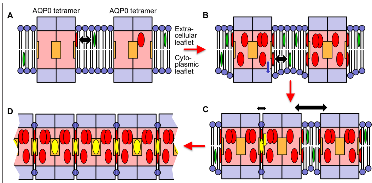
Figure 9. Proposed model for how an increasing cholesterol concentration drives aquaporin-0 (AQP0) two-dimensional (2D) array formation in the native lens membrane. (A) At a low cholesterol concentration, AQP0 tetramers are mostly surrounded by phospholipids and sphingomyelin. Free cholesterol in the membrane (green ovals) only associates with the highest affinity cholesterol-binding sites. Cholesterols occupying these peripheral binding sites are shown as red ovals and the black double-headed arrow indicates the transient nature of this interaction. The deep cholesterol-binding sites (orange squares) are not occupied. (B) With increasing cholesterol concentration, more cholesterols associate with the AQP0 surface. These cholesterols cause the interacting lipids in the cytoplasmic leaflet to move out from the bilayer center (blue arrow), resulting in the annular lipid shell that has a bigger hydrophobic thickness than the surrounding membrane, creating a hydrophobic mismatch that results in membrane deformation. (C) To minimize hydrophobic mismatch, AQP0 tetramers cluster. Cholesterol in between adjacent tetramers can move into the deep binding sites (yellow arrow) and cholesterol occupying deep binding sites (yellow ovals) act as glue that increases that association of the adjacent tetramers (indicated by the small double-headed black arrow) as compared to adjacent tetramers that do not sandwich a deep-binding cholesterol (indicated by the large double-headed black arrow). Clustering of proteins to minimize hydrophobic mismatch and stabilization by deep cholesterol-mediated protein–protein interactions may be the basis for the formation of transient lipid rafts. (D) Each AQP0 tetramer has four deep cholesterol-binding sites. As a result of the avidity effect, AQP0 can form large and stable 2D arrays.
