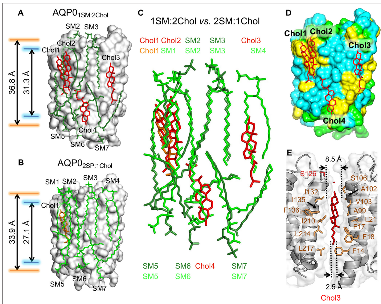
Figure 4. The 1:2 sphingomyelin/cholesterol bilayer surrounding aquaporin-0 (AQP0) and comparison with the 2:1 sphingomyelin/cholesterol bilayer. (A) The five sphingomyelins (dark green sticks) and four cholesterol (red sticks) molecules surrounding an AQP0 subunit (gray surface). The arrows between the orange and blue lines indicate the average distances between the phosphorus atoms of the phosphodiester groups and the nitrogen atoms of the amide groups in the two leaflets, respectively. (B) The AQP0 2SM:1Chol structure shown for comparison with the AQP0 1SM:2Chol structure in (A) . Arrows as in (A) . (C) Overlay of the lipid bilayers in the AQP0 2SM:1Chol and AQP0 1SM:2Chol structures. (D) Location of the four cholesterol (red sticks) in the AQP0 1SM:2Chol structure with respect to AQP0 surface characteristics. Color coding: yellow, aromatic residues; cyan, hydrophobic residues; and light green, polar and charged residues. (E) Position of cholesterol Chol3 (red sticks) in the AQP0 1SM:2Chol structure and its interaction with residues of two adjacent AQP0 tetramers (brown sticks). The dotted lines indicate the distance between the two adjacent AQP0 tetramers at the positions of the ring system (~8.5 Å) and the acyl chain (~2.5 Å). See also Figure 4—figure supplements 1 and 2 and Table 3 .
