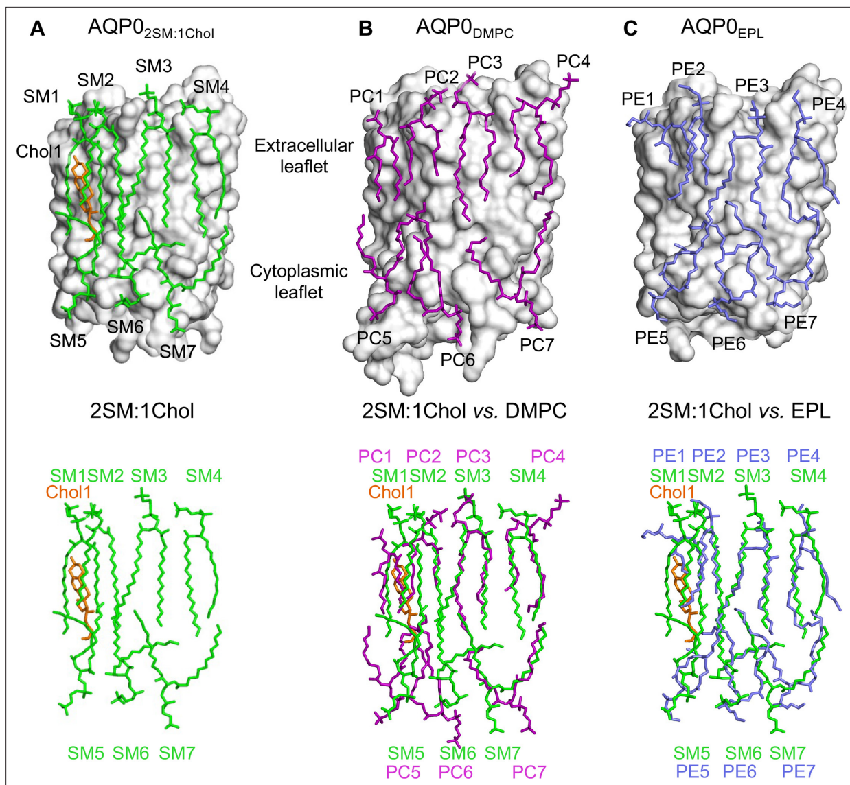
Figure 3. The 2:1 sphingomyelin/cholesterol bilayer surrounding aquaporin-0 (AQP0) is similar to bilayers formed by phosphoglycerolipids. (A) The top panel shows the seven sphingomyelins (light green sticks) and one cholesterol (orange sticks) molecules forming the bilayer around an AQP0 subunit (gray surface). The bottom panel shows just the lipid bilayer. (B) The top panel shows dimyristoyl phosphatidylcholine (DMPC) lipids (purple sticks) surrounding an AQP0 subunit (Gonen et al., 2005) and the bottom layer shows an overlay of the DMPC bilayer with the 2:1 sphingomyelin/cholesterol bilayer. (C) The top panel shows an Escherichia coli polar lipids extract (EPL) bilayer (modeled as PE lipids) (light brown sticks) surrounding an AQP0 subunit (Hite et al., 2010) and the bottom layer shows an overlay of the EPL bilayer with the 2:1 sphingomyelin/cholesterol bilayer. See also Figure 3—figure supplements 1–3 and Table 3 .
