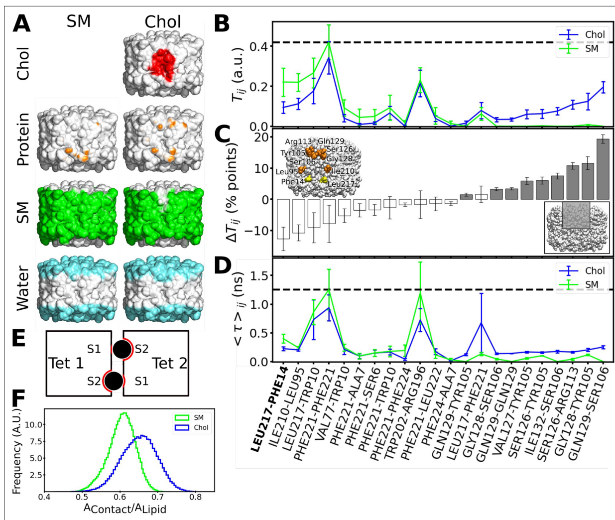
Figure 8. Interactions formed between adjacent aquaporin-0 (AQPO) tetramers and lipid-AQPO surface complementarity. (A) Equilibrium molecular dynamics (MD) simulations were performed with pairs of AQPO tetramers without cholesterol (left panels) or with cholesterol (right panels) at the interface. Density maps were calculated for different components next to the AQPO surface over time and these maps were projected onto the surface of one of the AQPO tetramers to represent their localization. For clarity, the second tetramer, which would be in front of the shown tetramer, is not shown. The density displayed at arbitrary density units is color-coded and shows the position of cholesterol (red), protein, i.e., the neighboring AQPO tetramer (brown), sphingomyelin (green), and water (cyan). (B) T_{ij} is defined as the fraction of time during which residues ( i, j ) from opposite tetramers are in contact. This quantity was extracted from the equilibrium simulations for the pure sphingomyelin interface T_{ij}(SM) and for the interface containing cholesterol T_{ij}(Chol) . T_{ij} = 0 means that i and j were never in contact and T_{ij} = 1 means that they were always in contact. (C) The pairwise difference \Delta T_{ij} = T_{ij}(Chol) - T_{ij}(SM) is shown, discarding insignificant changes ( \Delta T_{ij} < 1 percentage, %, points). Accordingly, a value of \Delta T_{ij} > 0 ( \Delta T_{ij} < 0 ) corresponds to protein-protein contacts that were more often observed in the simulations with cholesterol (sphingomyelin). For instance, the residue pair Gln129–Ser106 was observed almost 20 percentage points more time in the simulations with cholesterol. The color of the bars indicates the location of the residues (gray: inner part of the extracellular leaflet, i.e., where deep cholesterol resides; white: the rest of the interfacial protein surface, see inset at lower right). Residues involved in a high \Delta T_{ij} > 10 percentage points are highlighted in orange in the inset (yellow for the contact Leu217–Phe214 observed in the electron crystallographic structure). (D) The average duration for every established protein–protein contact, \langle \tau \rangle_{ij} , is also displayed for the two different lipid interfaces. In (B) and (D) , the horizontal dashed lines indicate the highest value observed for all possible residue pairs. Contacts observed in the electron crystallographic structures are highlighted in bold letters. In B–D, the avg \pm s.e.m. is presented ( n=20 , i.e. 10 independent simulation times with two symmetric monomeric interfaces). (E) The schematic drawing depicts a top view of the two associated AQPO tetramers (squares, ‘Tet 1’ and ‘Tet 2’) with the two central lipids sandwiched between them (black circles). The other lipids at the interface are not shown for clarity. The respective monomer surfaces S1 and S2 are indicated. The region of the surface of the two tetramers that is in total covered by a lipid, A_{Contact} (red line) was normalized by the surface area of the lipid, A_{Lipid} (here corresponding to the perimeter of the circles). This ratio gives a measure of the surface complementarity between the tetramers and the sandwiched lipids, i.e., the higher the value of A_{Contact}/A_{Lipid} the more the two surfaces complement each other. (F) Normalized histograms of A_{Contact}/A_{Lipid} obtained from the equilibrium MD simulations are shown for the central sphingomyelin (SM) and cholesterol (Chol). See also Figure 8—figure supplements 1–3 .
