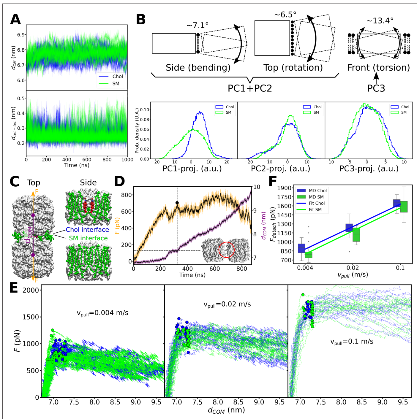
Figure 7. Equilibrium molecular dynamics (MD) simulations of pairs of associated aquaporin-0 (AQP0) tetramers and force-induced separation of two associated AQP0 tetramers. (A) Distance between the centers of mass d_{COM} (top) and minimum distance d_{tet-tet} (bottom) between the pair of AQP0 tetramers during the 2x AQP0 simulations in equilibrium for the interface containing only sphingomyelin (SM) molecules (SM, green) and the interface containing the deep cholesterol (Chol, blue) ( n=10 simulations for each case). (B) Principal component (PC) analysis of the relative movements between the two tetramers. Here, the motion of one of the tetramers (dashed-line rectangle) relative to the other tetramer (solid-line rectangle) was monitored. The three main PC accounted for 67.9% of the total relative motion between tetramers (PC1: 34.3%, PC2: 24.7%, and PC3: 8.9%). The schematic drawings illustrate the three main modes of motion: bending (depicted in the drawing as viewed from the side of the membrane), lateral rotation (depicted in the drawing as viewed from the top of the membrane), and torsion (depicted in the drawing as viewed from the side of the membrane with one tetramer in front of the other). Lipids at the interface between the two tetramers (first two panels) and lipids surrounding the two tetramers (last panel) are shown. PC1 plus PC2 capture the bending and rotation while PC3 corresponds to torsion. The histograms in the bottom panels show the projections of the MD trajectories onto the three main PC vectors, for the interfaces containing only sphingomyelin (SM, green) or containing the
