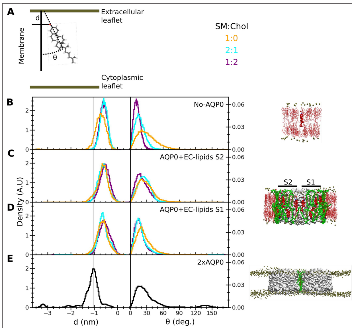
Figure 6. Insertion depth and orientation of a cholesterol at the interface between two aquaporin-0 (AQP0) tetramers. (A) Schematic figure illustrating how the insertion depth, d , and orientation angle, \theta , of the cholesterol were measured. The cholesterol insertion depth was defined as the distance in z direction of the cholesterol oxygen atom (red stick representation) from the center of mass of the phosphorus atoms of the nearby sphingomyelin (SM) molecules in the extracellular leaflet (top green horizontal line). The cholesterol orientation was defined as the angle between the membrane normal (simulation box z -vector) and the vector along the rings of the cholesterol molecule (black dashed line). (B–E) Right panels: The three different systems that were simulated, namely (B) 'No AQP0', a pure lipid membrane without AQP0, (C, D) 'AQP0+EC lipids S2/1', a membrane with one AQP0 tetramer surrounded by the annular lipids seen in the AQP0 1SM:2Chol structure, and (E) '2xAQP0', a membrane containing a pair of AQP0 tetramers together with the lipids in between them from a hybrid AQP0 2SM:1Chol structure that replaces the two central SM molecules with the EC deep cholesterol molecules found in the AQP0 1SM:2Chol structure. Left panels: Graphs showing normalized histograms for the insertion depth, d , and orientation angle, \theta , for the monitored deep cholesterol in membranes with different SM:Chol ratios (see color code in panel A ), except for the 2xAQP0 system, which was only simulated in a pure SM membrane. For the simulations with one AQP0 tetramer, insertion and orientation were computed separately for the deep cholesterol located at surface S2 ( C ) and S1 ( D ). The vertical line indicates the most probable cholesterol position in the 2xAQP0 system ( E ). See also Figure 6—figure supplement 1 .
