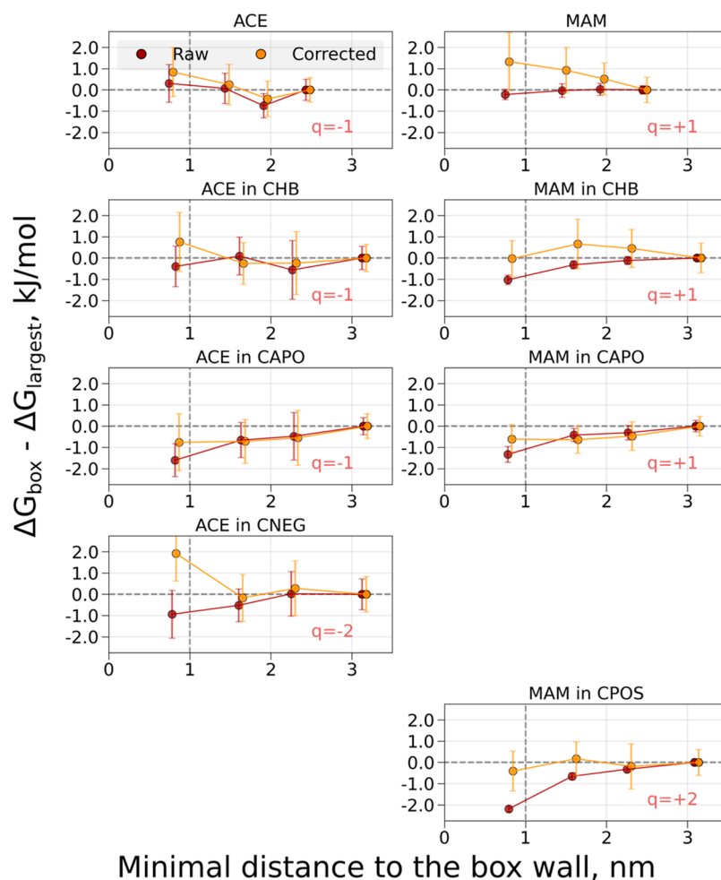
Figure 5. Free-energy differences and corrections for coupling electrostatic interactions of the ACE and MAM ligands and decoupling/coupling an ion in solution in systems with 0.5 M salt. The charge modifications were performed to retain a constant overall charge of the simulation box. The topology setup retaining a constantly charged box was used. The system was solvated in water and 0.5 M salt (sodium and chloride) was added. Simulations were performed in cubic boxes of varying sizes: the x -axis denotes the minimal distances for the buckyball-solute to the cell wall for every box size; the values on the y -axis denote \Delta G differences between the values obtained in the individual box and the largest considered box. The darker-colored symbols indicate raw calculated free energies, while the light-colored symbols mark the free-energy values with the corrections added. The symbols for the corrected values are offset by 0.05 nm along the x -axis for visualization purposes.
