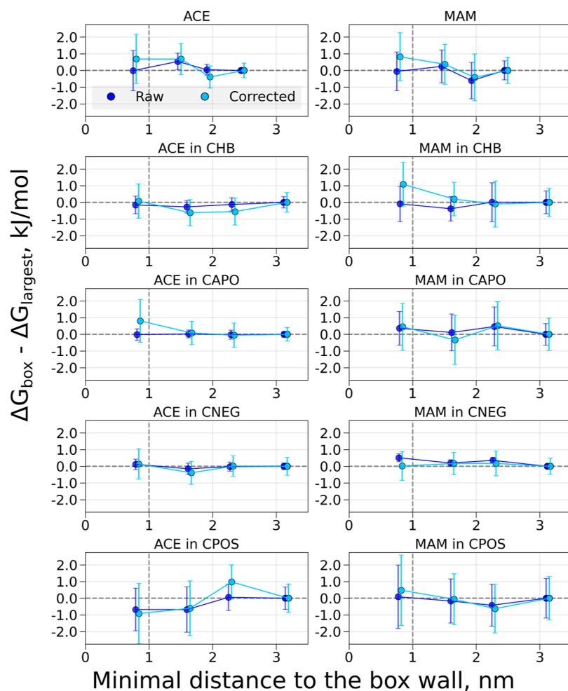
Figure 6. Free-energy differences and corrections for coupling electrostatic interactions of the ACE and MAM ligands and decoupling/coperturbing an ion in solution in systems with 0.5 M salt. The charge modifications were performed to retain a constant overall charge of the simulation box. The topology setup retaining a neutral simulation box was used. The system was solvated in water and 0.5 M salt (sodium and chloride) was added. Simulations were performed in cubic boxes of varying sizes: the x -axis denotes the minimal distances for the buckyball-solute-ion to the cell wall for every box size; the values on the y -axis denote \Delta G differences between the values obtained in the individual box and the largest considered box. The darker-colored symbols indicate raw calculated free energies, while the light-colored symbols mark the free-energy values with the corrections added. The symbols for the corrected values are offset by 0.05 nm along the x -axis for visualization purposes.
