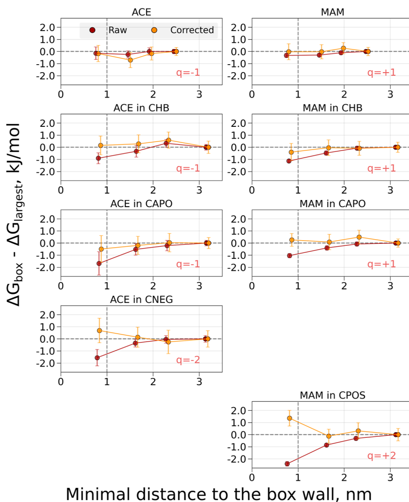
Figure 3. Free-energy differences and corrections for coupling electrostatic interactions of the ACE and MAM ligands and decoupling/coperturbing an ion in solution. The charge modifications were performed to retain a constant overall charge in the simulation box. The topology setup retaining a constantly charged box was used. The systems were solvated in water, and no additional salt was added. Simulations were performed in cubic boxes of varying size: the values on the x -axis denote the minimal distances for the buckyball-solute-ion to the cell wall for every box size; the values on the y -axis denote the \Delta G differences between the values obtained in the individual box and the largest considered box. The darker-colored symbols indicate raw calculated free energies, while the light-colored symbols mark the free-energy values with the corrections added. The symbols for the corrected values are offset by 0.05 nm along the x -axis for visualization purposes.
